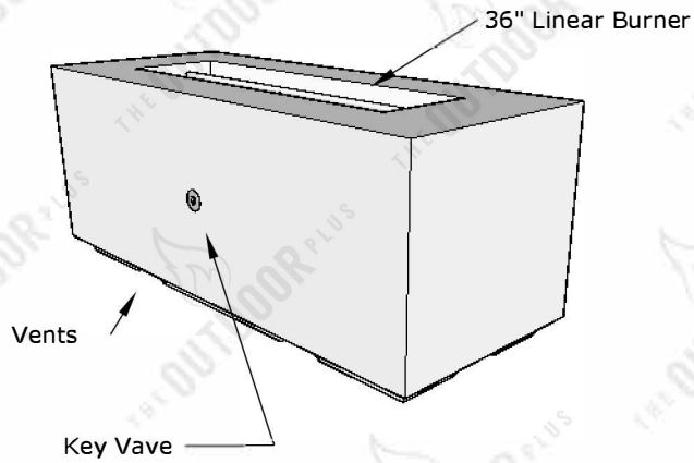
PERSPECTIVE
